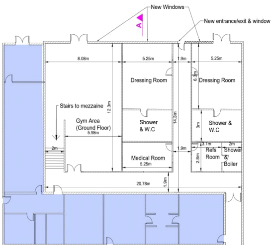
SECTIONAL PLAN VIEW Scale 1:100@A1
